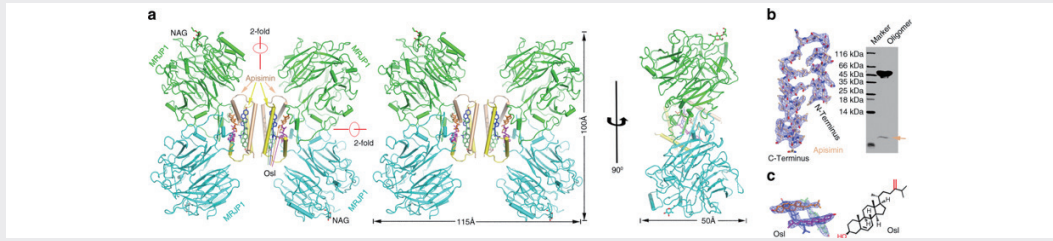
▲ Structure of the MRJP1 oligomer
